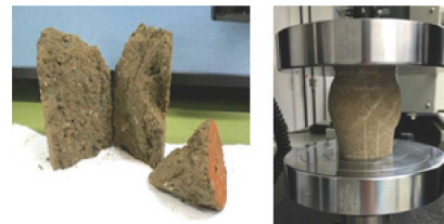
(Comparison of cemented soil and composite material) Fig.2 Improvement of earthquake resistance of underground structure using new composite ground material
