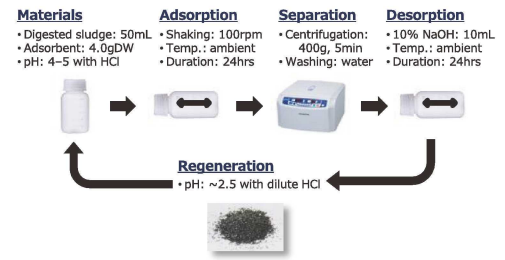
Fig.3 Procedure for phosphate adsorption
