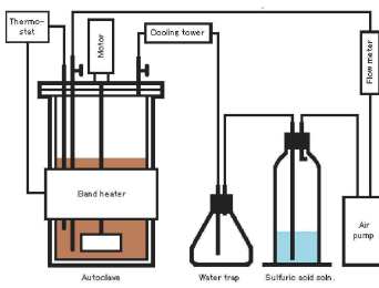
Fig.2 Ammonia stripping device
