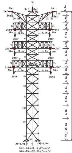
Fig.3 Initial configuration of a transmission tower truss
